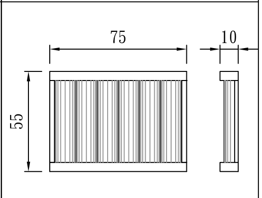
型號：DF-W75T10H55
