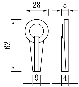
型號：DF-W28T8H62
